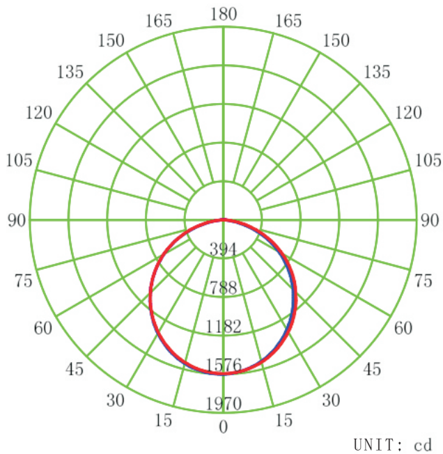
LUMINOUS INTENSITY DISTRIBUTION DIAGRAM
